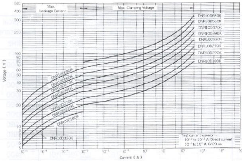
V-I Curve DNR10D180K to DNR10D680K
