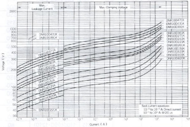
V-I Curve DNR10D820K to DNR10D471K
