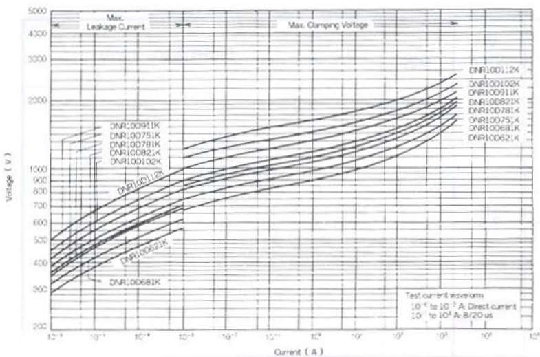
V-I Curve DNR10D621K to DNR10D112K
