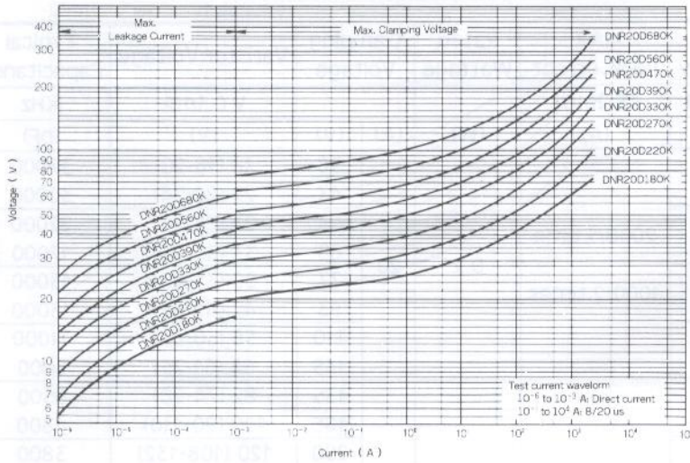
V-I Curve DNR20D180K to DNR20D680K
