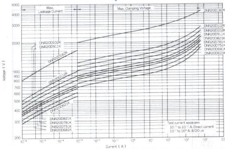
V-I Curve DNR20D621K to DNR20D182K
