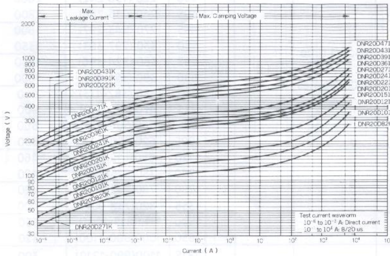
V-I Curve DNR20D820K to DNR20D471K
