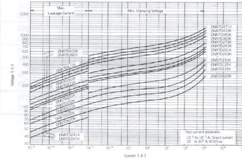
V-I Curve DNR7D820K to DNR7D471K
